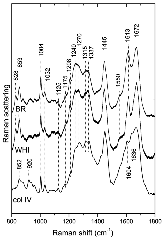
Fig. 4. FT-Raman spectra of white (WHI) and brown (BR) G. melastomus egg case specimens and collagen IV (col IV). Peaks are labelled as scattering maxima. The spectra have been offset for clarity.
